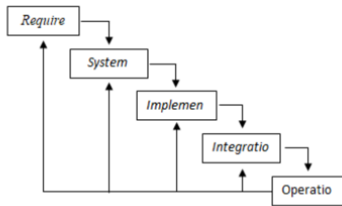
Gambar 1 Metode Waterfall
