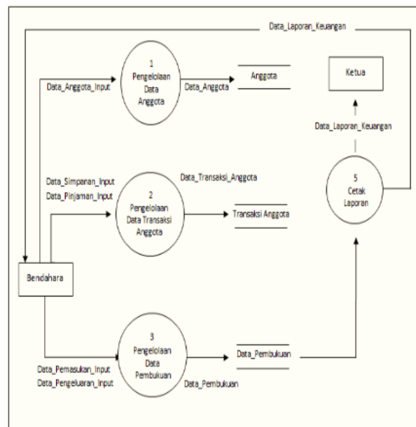
Gambar 9 Data Flow Diagram Level 1
